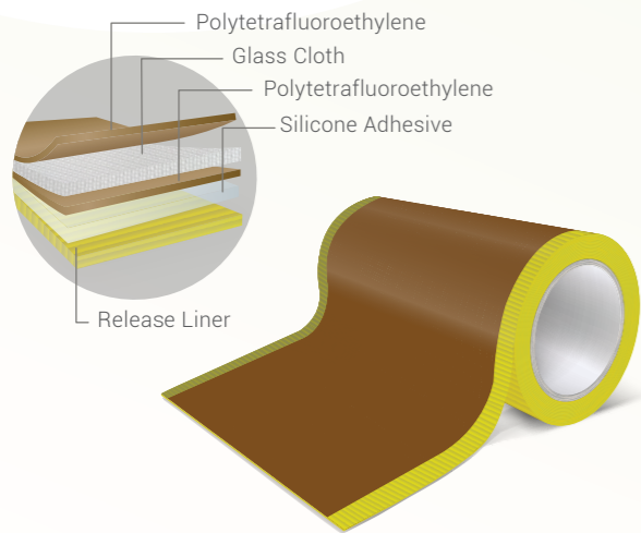
High Temperature (PTFE) PTFE Cloth with Liner
