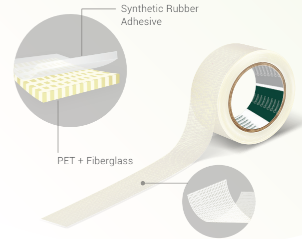
Filament Tape
