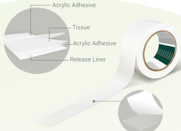
Nonwoven Double Sided Non-woven Tape
