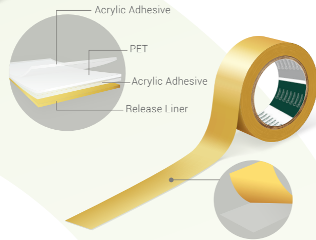
Filmic Double Sided PET Tape
