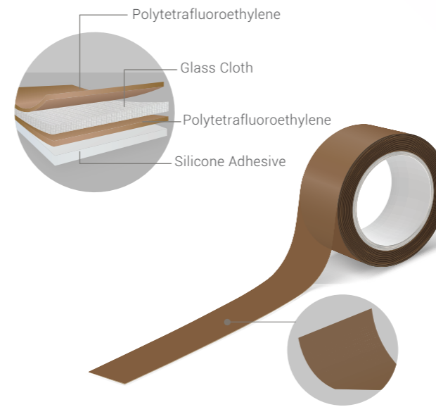
High Temperature (PTFE) PTFE Tape
